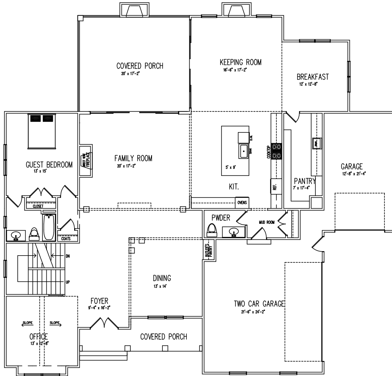
PRESERVE 1 MAIN FLOOR PLAN
